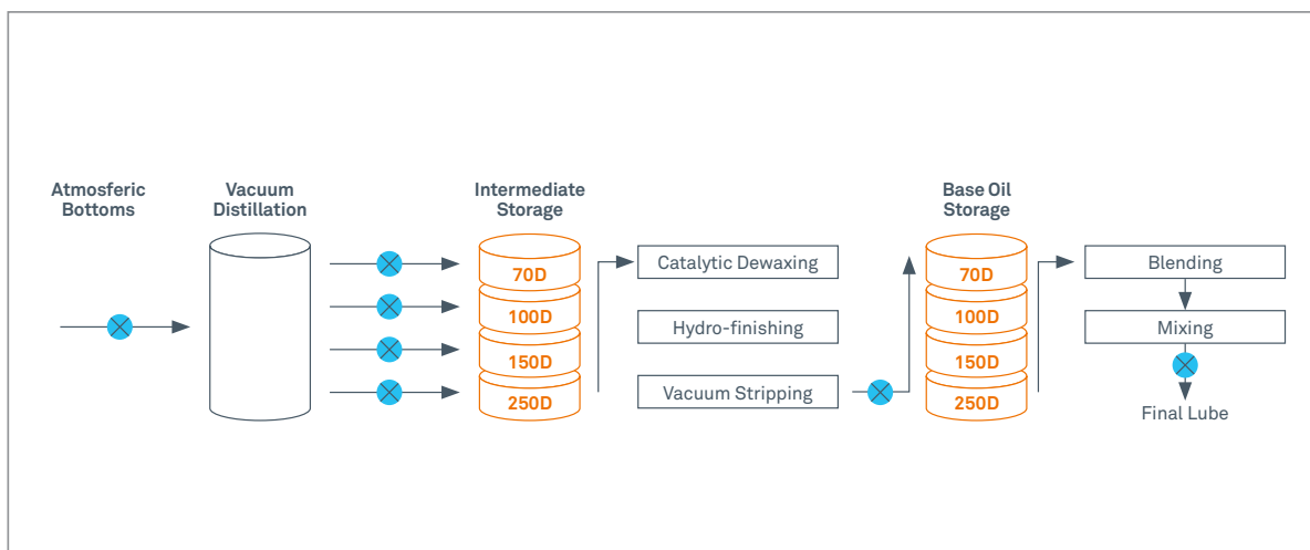
Fig. 3: Optimal viscosity measurement locations (●) for an efficient and high-quality lube production.
