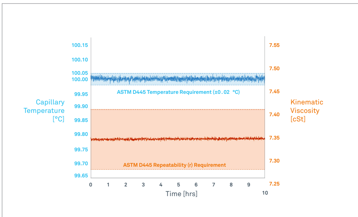
Fig. 2: Kinematic viscosity readings and capillary temperature of an engine oil sample (5W20) with the BENKE VISC-4 at 100 °C. The ASTM D445 repeatability (r) and temperature range of \pm 0.02 °C are highlighted.
